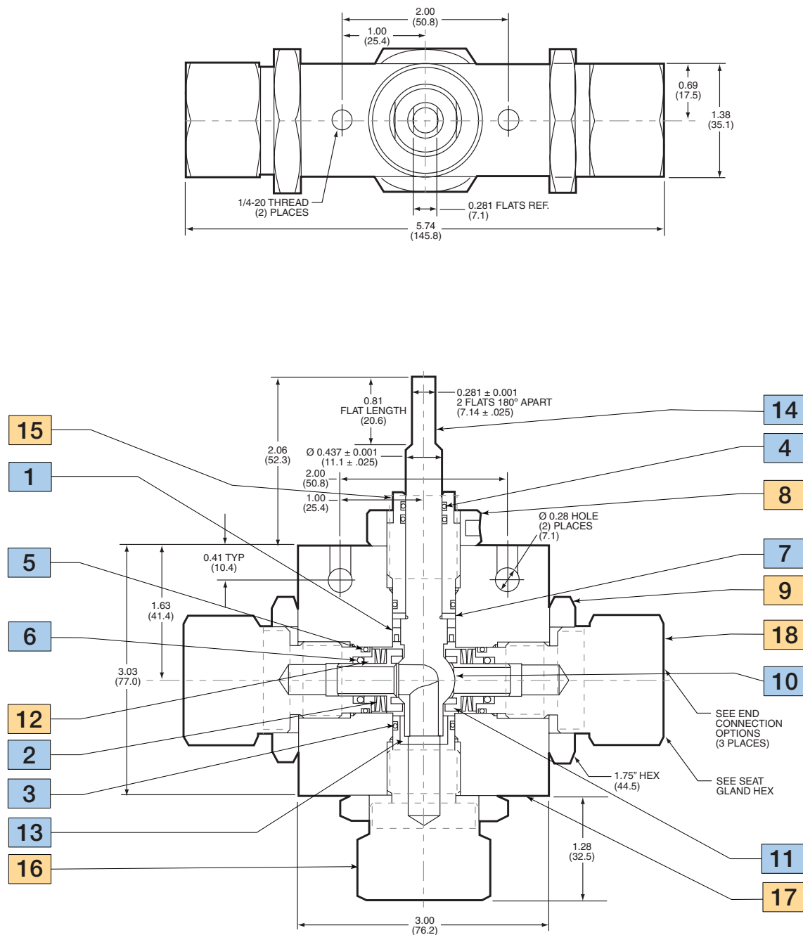
1/2" 3 Way Subsea Ball Valve
